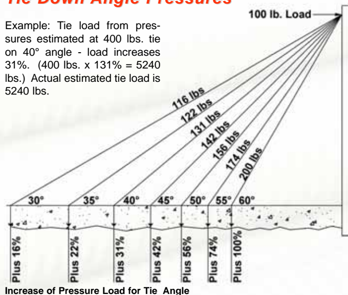
Increase of Pressure Load for Tie Angle
