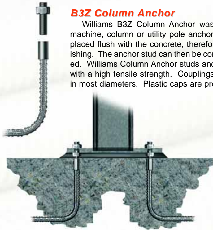
Steel Column Anchor
